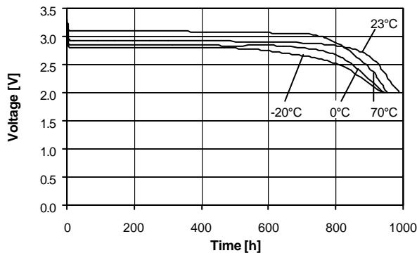
Temperature performance Load 12kW
